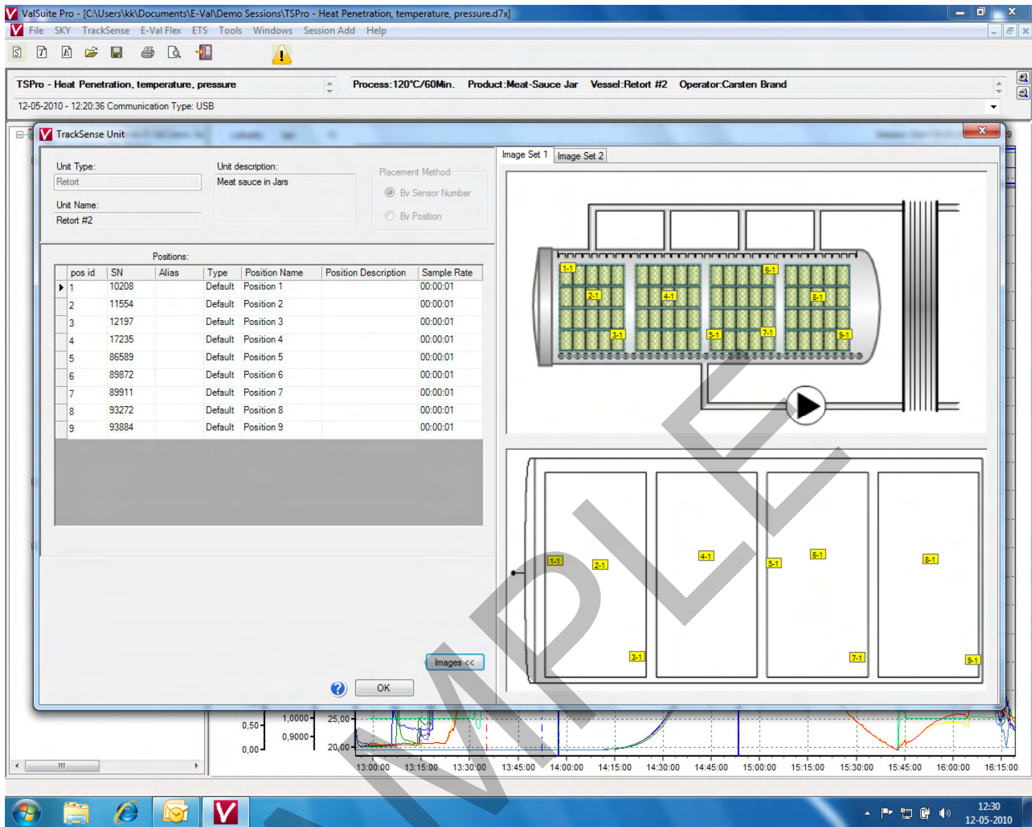
Example of probe positioning in a Retort. Channel numbers are easily positioned on photos or drawings.
