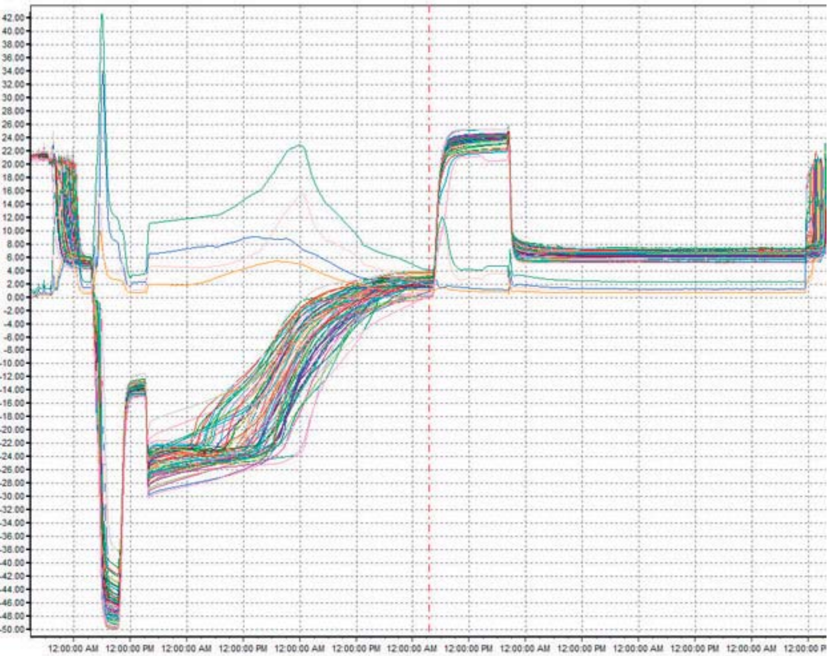
This ValSuite™ graph illustrates a typical temperature profile of a Lyophilization process. Data is collected using 40 TrackSense® Pro loggers with a total of 80 measuring points.
